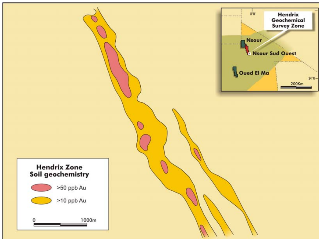
Hendrix Zone gold anomaly, Nsour Sud Ouest application
