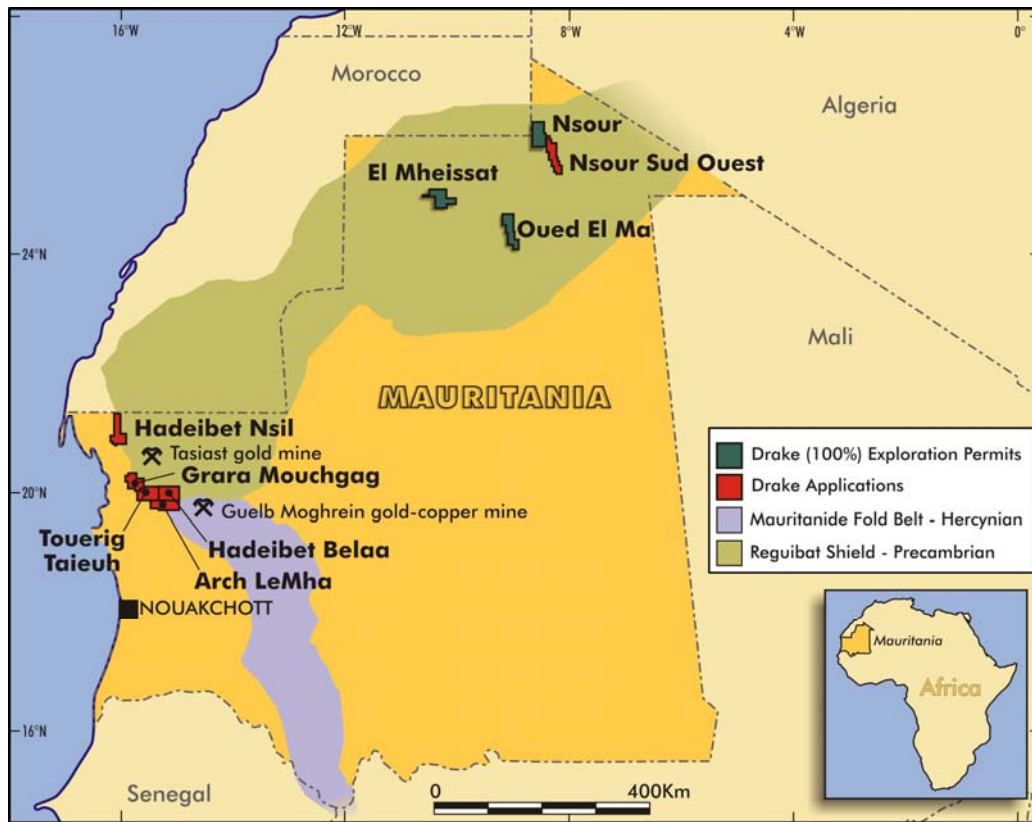
Location of Drake Resources' gold permits and applications in Mauritania
