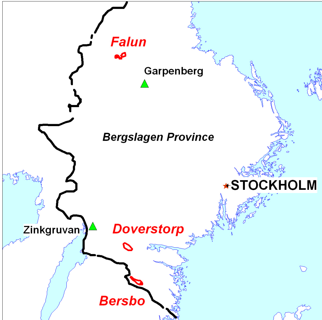
Location of the detailed airborne surveys in Sweden in red
